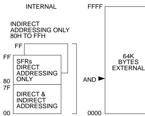
Figure 6. The 80C52, 83C154 and 83C154D Data Memory Organisation.
