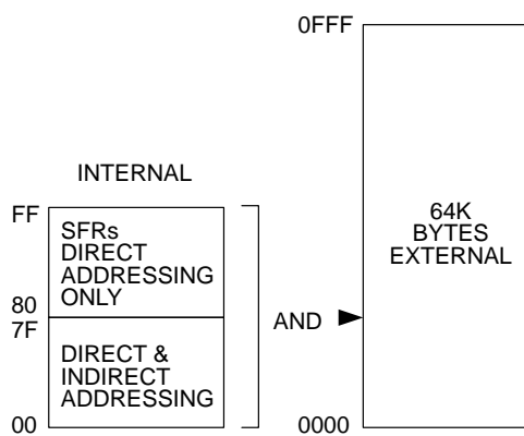
Figure 5. The 80C51 Data Memory Organisation.
